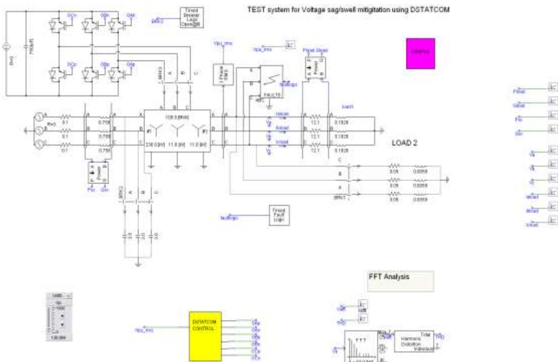
Fig.4 (a) PCSAD/EMTDC model of a three phase 6-pulse.
