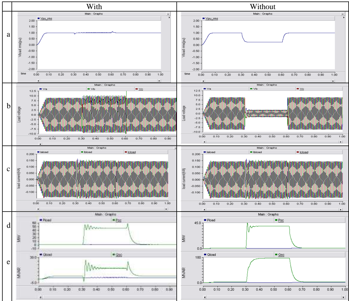
Fig.5 Waveforms for a voltage of 81% (a) rms load voltage (pu) (b) Instantaneous load voltages (kV) (c) Instantaneous load currents (kA) (d) Load and source active powers (MW) (e) Load and source reactive power (MVAR)
