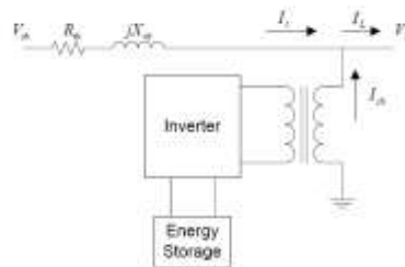
Fig3.Schematic of D-STATCOM
